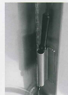
High-quality components: the core and chamber temperatures are measured with the proven PT 100 sensor from FESSMANN.
